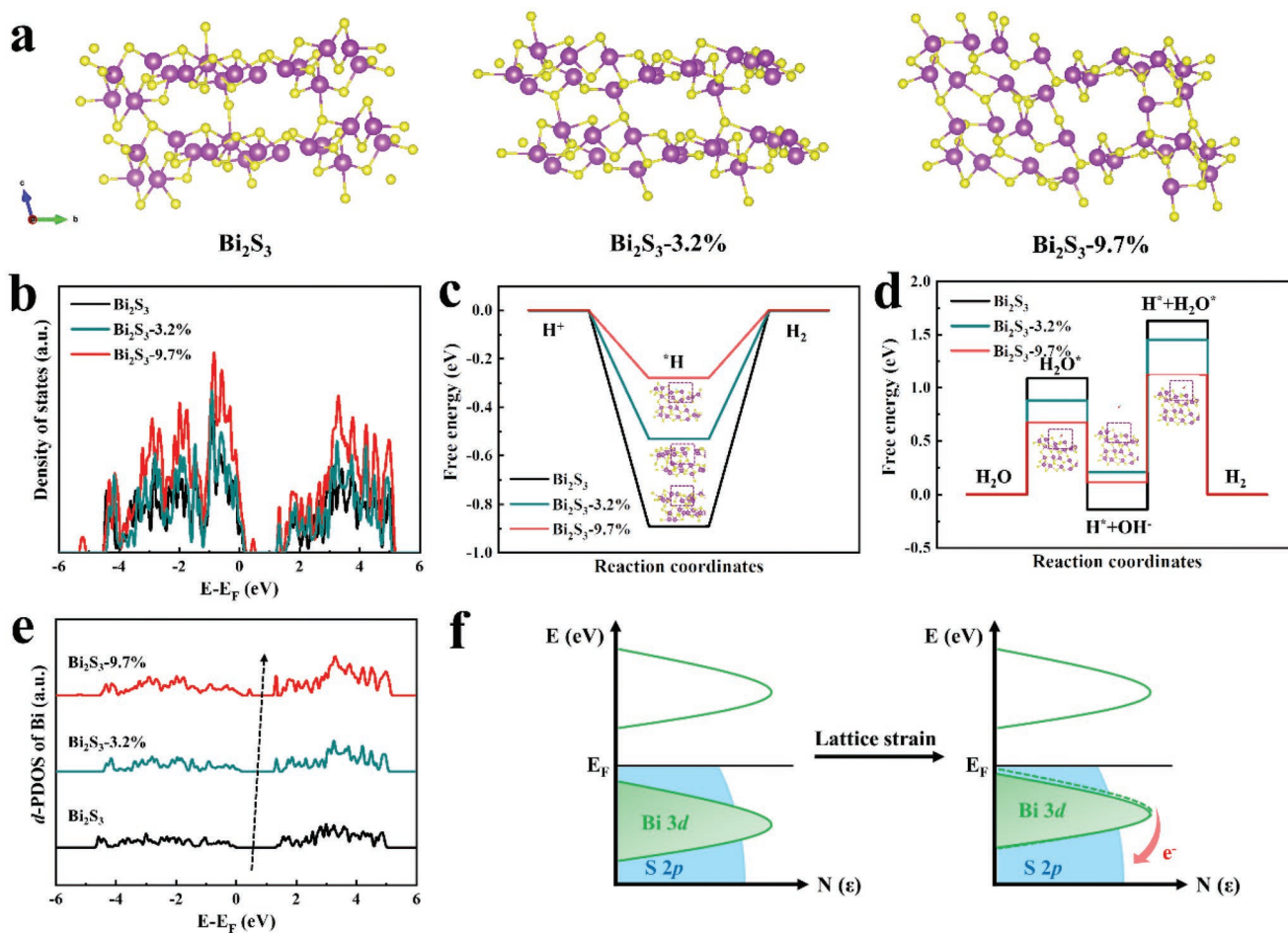
Figure 5. Interpretation of the lattice strain on the influence of HER activity. a) The geometric structures and b) electronic structure of Bi 2 S 3 samples with different lattice strains. c) The optimized structures and Gibbs free energy diagrams of HER in an acidic medium. d) The optimized structures and Gibbs free energy diagrams of HER in alkaline and neutral media. e) The d-orbital partial density of states ( d -PDOS) of Bi in the Bi 2 S 3 samples. f) Schematic of the electron exchange for Bi 2 S 3 -9.7%.
