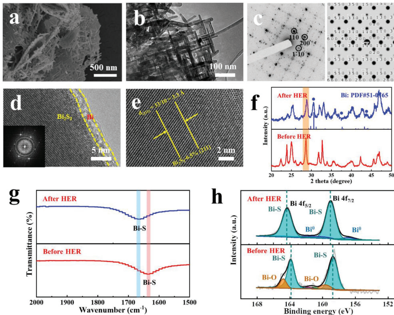
Figure 6. Active sites for hydrogen evolution catalysis. a) SEM, b) TEM, c) corresponding SAED pattern (left) and simulated SAED pattern (right) of \text{Bi}_2\text{S}_3 -9.7% after HER in alkaline solution. d,e) HRTEM of \text{Bi}_2\text{S}_3 -9.7% after HER in alkaline solution (Inset: corresponding SAED pattern). f) XRD patterns of \text{Bi}_2\text{S}_3 -9.7% before and after HER in alkaline solution. g) FT-IR spectra of \text{Bi}_2\text{S}_3 -9.7% before and after HER in alkaline solution. h) XPS of \text{Bi}_2\text{S}_3 -9.7% before and after HER in alkaline solution. All the spectra were shown with raw data and fitting data derived by Lorentz–Gaussian function.
