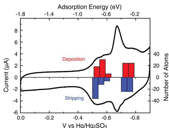
Fig. 2 A CV showing the Pb UPD process at a \text{Au}_{147} DEN-modified glassy carbon electrode. The scan rate was 5 mV s -1 and the aqueous electrolyte solution contained 1.0 mM \text{Pb}(\text{NO}_3)_2 in 0.10 M \text{HClO}_4 . The DFT-calculated potentials for Pb deposition (red bars) and stripping (blue bars) are also shown.
