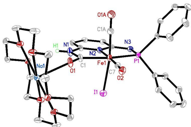
Figure 3. ORTEP diagram (30% thermal ellipsoids) for [Na(18-crown-6)][[(C NH N=P Ph 2 )Fe(CO) 2 ]] ( 7 ). H atoms except for the NH proton are omitted for clarity.
