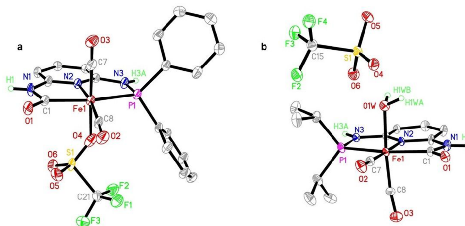
Figure 1. ORTEP diagrams for (a) [(C^{NH}N^{NH}P^{Ph_2})Fe(CO)_2(OTf)] ( 3 ) (30% thermal ellipsoids) and (b) [(C^{NH}N^{NH}P^{iPr_2})Fe(CO)_2(H_2O)](OTf) ( 4-H 2 O ) (50% thermal ellipsoids). The H atoms except for the NH protons are omitted for clarity.
