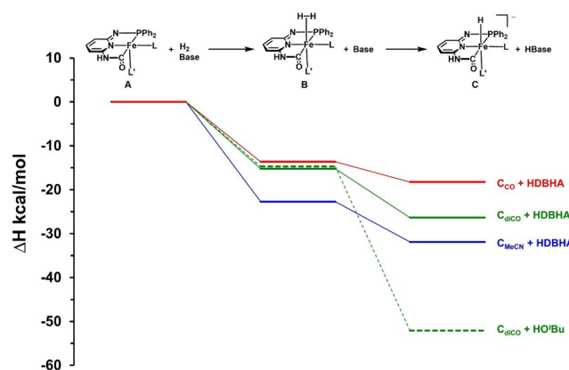
Figure 9. Calculated relative enthalpies in the H 2 binding and cleavage reactions with external bases of A CO + NaDBHA (red), A diCO + NaDBHA (solid green), A MeCN + NaDBHA (blue) and A diCO + KO t Bu (dashed green) proceeding from the corrected iso-energetic state A through B and forming C .
