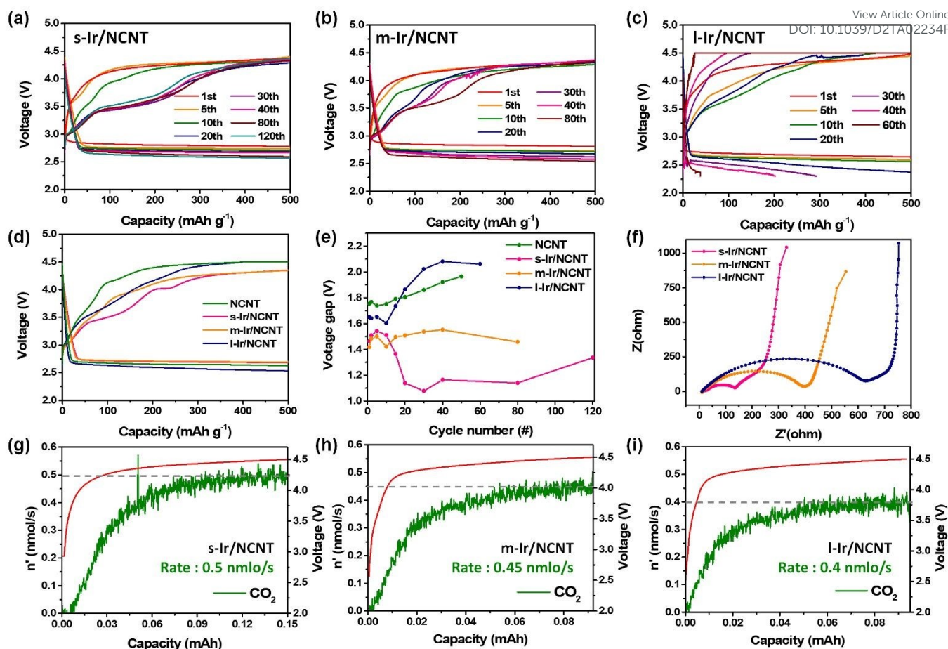
Fig. 5 Electrochemical cell data of NCNT, s-, m- and l-Ir/NCNTs: (a–c) Cycling performance of Li-CO 2 cells fabricated using s-, m-, and l-Ir/NCNTs loaded electrodes measured at 50 mA g carbon -1 with limited capacity of 500 mAh g carbon -1 . (d) Discharge/charge curves during the 15th cycle. (e) Voltage gap graphs calculated during the discharge and charge reactions for Li-CO 2 cells at 250 mAh g -1 during each cycle. (f) EIS of the s-, m- and l-Ir/NCNT-containing electrode after 10 cycles. (g–i) in situ DEMS results of gas evolution rate for CO 2 during charging in cells with s-, m- and l-Ir/NCNTs.
