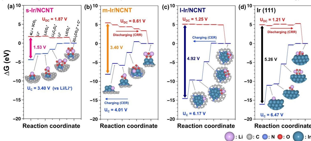
Fig. 6 Reaction energy diagram of charging and discharging for Li- \text{CO}_2 battery on (a) s-Ir/NCNT, (b) m-Ir/NCNT, (c) l-Ir/NCNT, and (d) Ir (111) surface.
