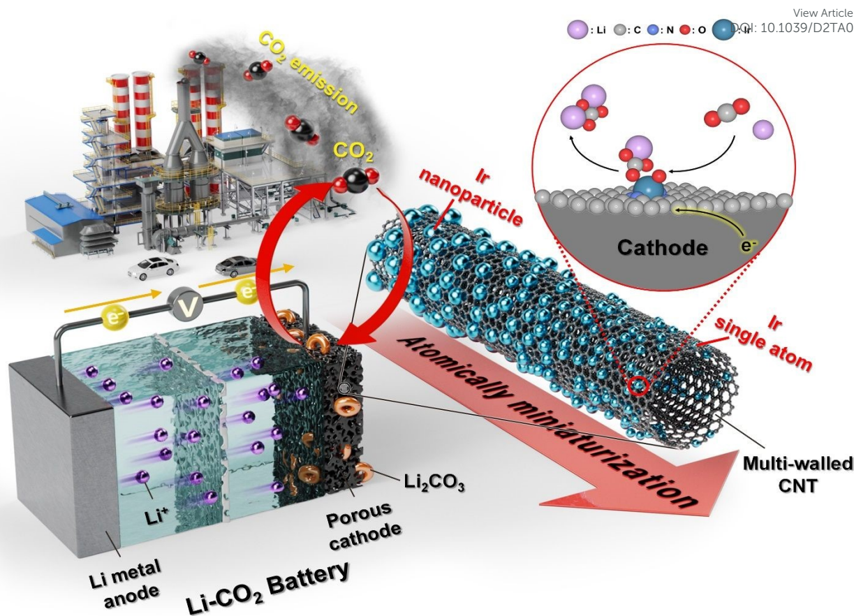
Fig. 1 Schematic illustration of Li-CO 2 battery employing atomically minimized IrO x /Ir bi-phase catalysts and the mechanism through which they catalyze the Li-CO 2 reaction.
