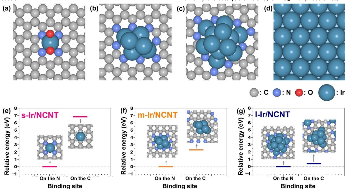
Fig. 4 Illustrations of structures representing the s-, m-, and l-Ir particles on the NCNT: (a) IrO 2 SAC for small particles, (b) Ir 6 NP for medium-sized particles, (c) Ir 12 NP for large NPs, and (d) Ir (111) surface for comparison. Relative binding energies of (e) Ir atom, (f) Ir 6 , and (g) Ir 12 NP on the NCNTs.
