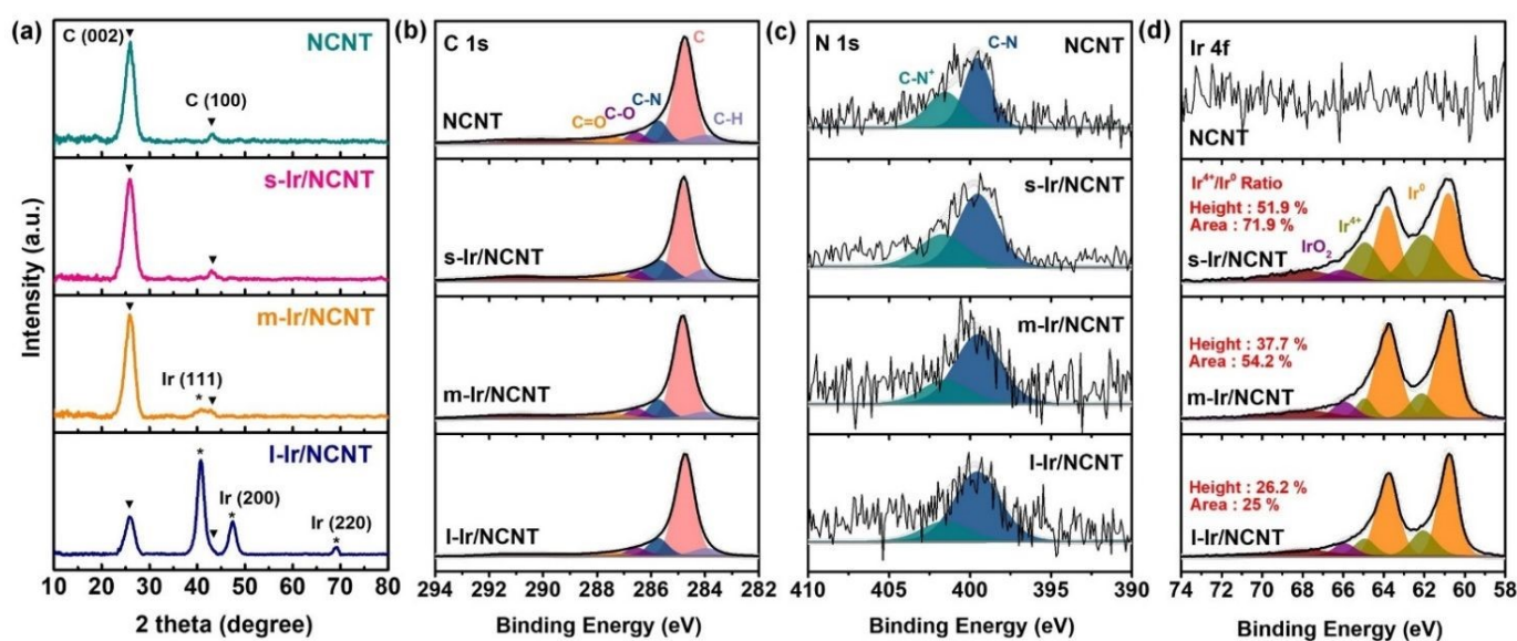
Fig. 3 Structural and chemical characterization of NCNT, s-, m- and l-Ir/NCNTs: (a) XRD patterns; (b) C 1s, (c) N 1s, and (d) Ir 4f XPS spectra.
