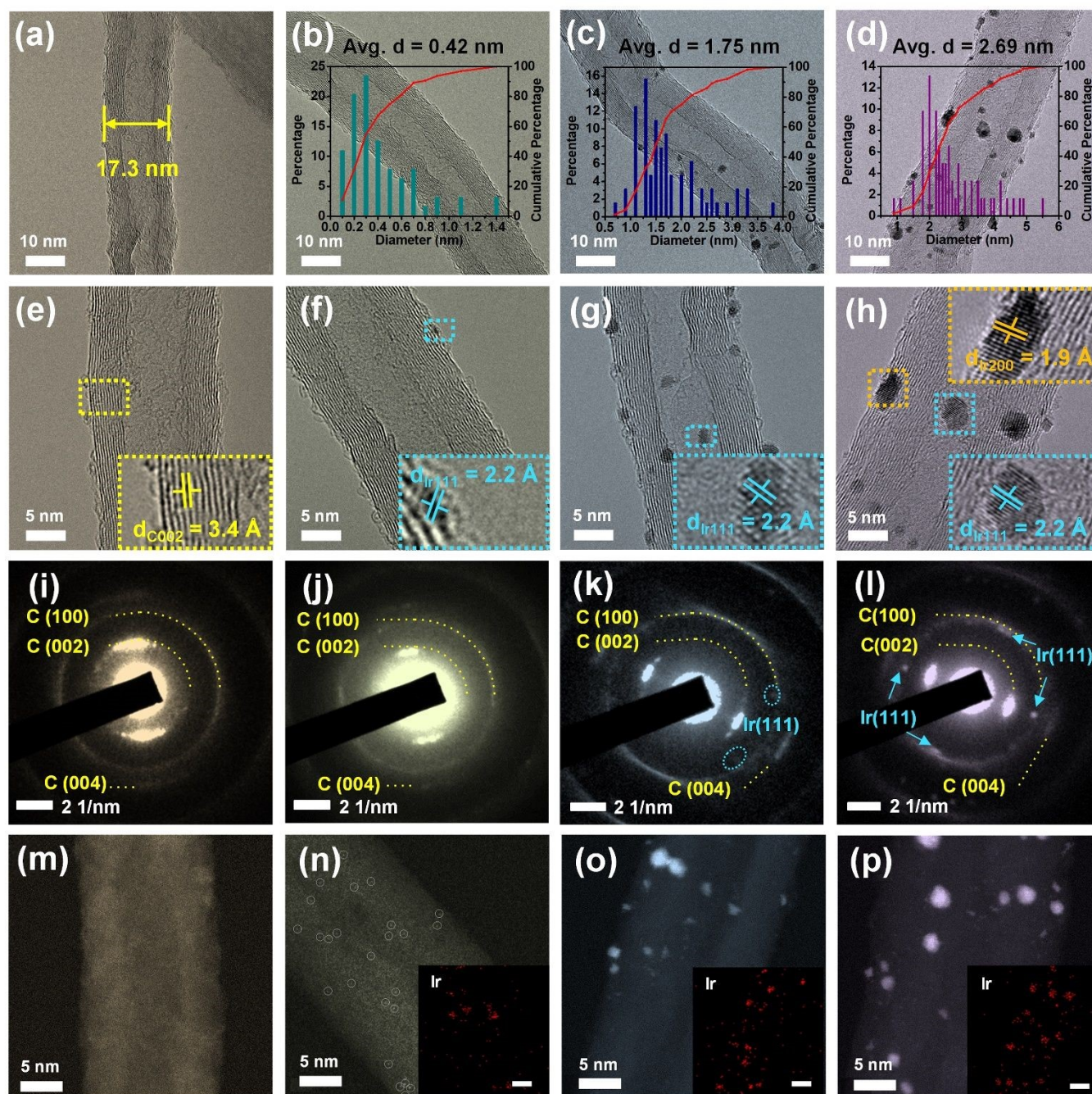
Fig. 2 Morphologic characterization of NCNT (a, e, i, m); s-Ir/NCNT (b, f, j, n); m-Ir/NCNT (c, g, k, o) and l-Ir/NCNT (d, h, l, p): (a–h) TEM images, (i–l) SAED patterns, (m–p) STEM and (insets of n–p) EDS elemental maps. The insets of Figs. 2b–d demonstrate the relatively uniform Ir particle distribution of each sample.
