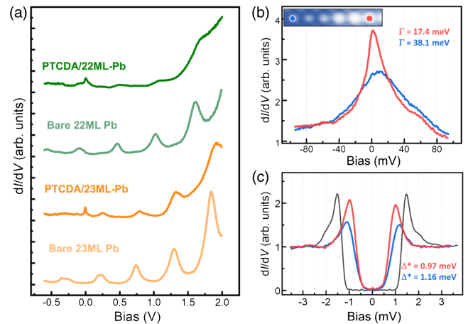
FIG. 4. (a) dI/dV spectra from -0.6 to +2.0 V taken on the ML PTCDA/22 ML Pb, bare 22 ML, ML PTCDA/23 ML Pb, and 23 ML Pb surfaces. (b) and (c) Measurements of Kondo resonances and pairing gaps on ML PTCDA/22 ML Pb. Two typical spots are chosen: the morphologically highest (red) and lowest (blue) molecules within one moiré periodicity [labeled in the inset of (b)]. The black curve in (c) is taken on bare 22 ML Pb with its SC gap \Delta_0^{22 \text{ ML}} = 1.35 \text{ meV} [21]. All spectra were taken at 0.4 K with a normal tip. (b) V_s = 95 \text{ mV} , I = 100 \text{ pA} , and V_{\text{rms}} = 2.5 \text{ mV} ; (c) V_s = 3.5 \text{ mV} , I = 100 \text{ pA} , and V_{\text{rms}} = 50 \mu\text{V} .
