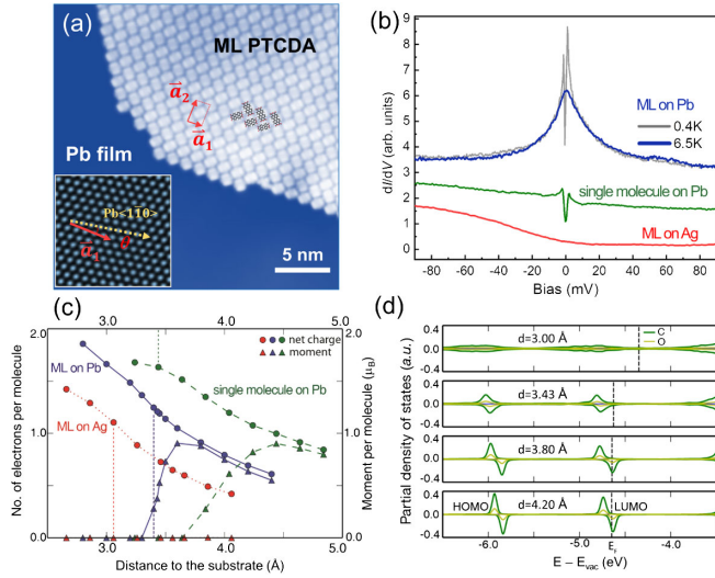
FIG. 1. (a) STM image of ML PTCDA/Pb film. The red rectangle represents a unit cell of the herringbone structure. The inset shows the atomically resolved image of the nearby Pb surface ( 4 \times 4 \text{ nm}^2 ). The twist angle \theta is defined as labeled. (b) dI/dV spectra for the ML PTCDA/Pb, T_S = 0.4 K (gray) and 6.5 K (blue), a single molecule on Pb at 0.4 K (green), and the ML PTCDA on Ag(111) at 4.2 K (red). Spectra are shifted vertically for clarity. (c) The charge transfer and the magnetic moment as a function of the d for all three situations. The equilibrium distances are marked by vertical dashed lines. (d) Partial DOS at various d for ML PTCDA/Pb. The dashed lines indicate the Fermi levels (a) Sample bias V_S = 1.0 V, setpoint current I = 25 pA. Setpoint in (b): V_S = 95 mV, I = 200 pA, and the lock-in modulation V_{\text{rms}} = 0.8 mV.
