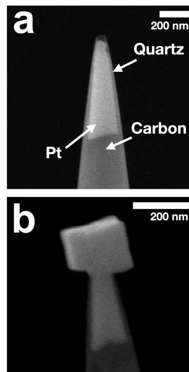
Figure 2. SEM images of a CNE (a) after the initial stage of Pt electrodeposition in which only the recessed portion of the CNE has been filled and (b) after the second stage of Pt electrodeposition in which a Pt NP (TPH, in this case) forms atop the electrode.
