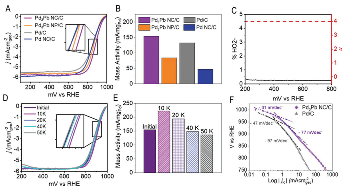
Fig. 3 (A) Polarization curves collected in O 2 -saturated 0.1 M KOH and (B) corresponding mass activities. (C) RRDE results for the determination of % HO 2 - and n for Pd 3 Pb NC/C. (D) Polarization curves collected in O 2 -saturated before and after ADT and (E) mass activities after ADT at different intervals for the Pd 3 Pd NC/C. (F) Tafel plots for Pd 3 Pb NC/C compared to the Pd/C.
